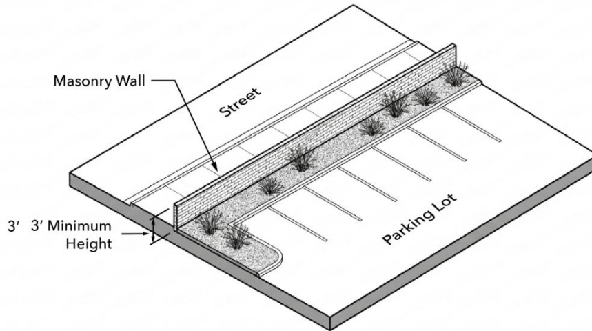
Figure 4.36.1B: Parking Area Screening
