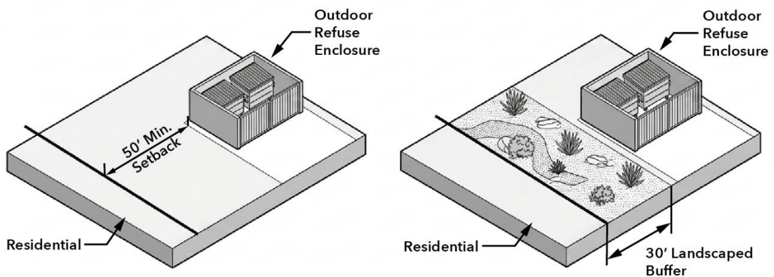
Figure 4.6.1C -- Outdoor Refuse Screening
