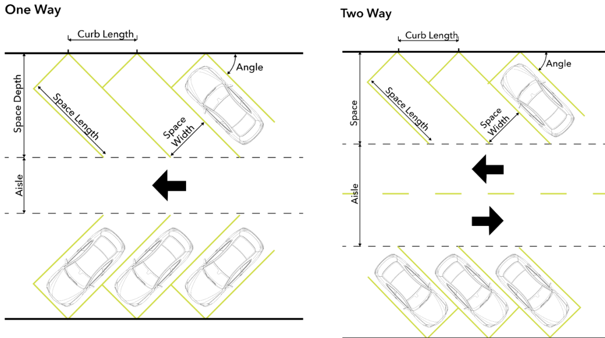
Figure 4.4.3B3 - Parking and Aisle Dimensions
