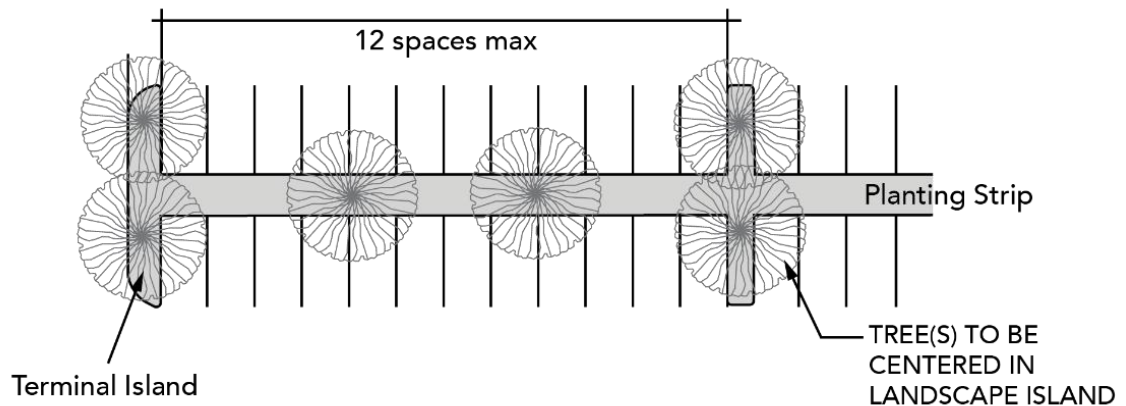
Figure 4.25.4A - Parking Area Landscaping
